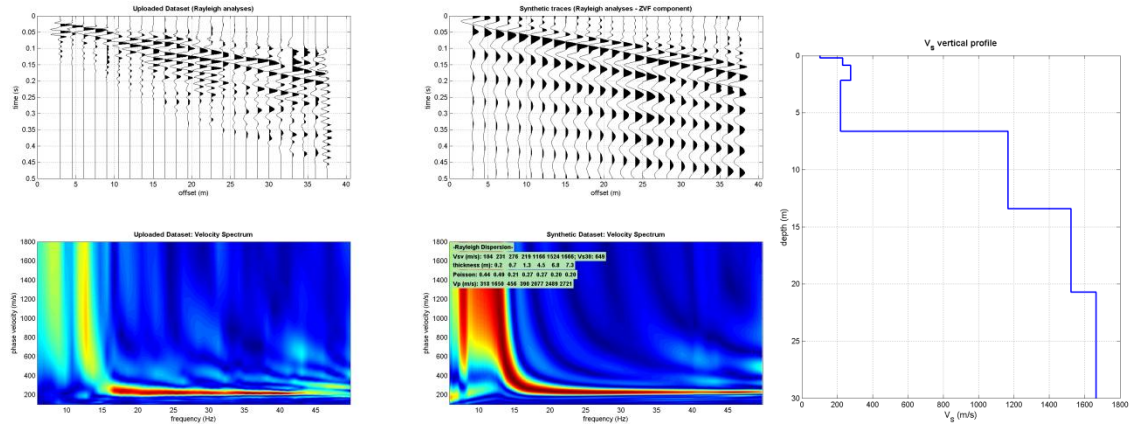
Figure 6. Full waveform interpretation results from site 1 in figure 2.
