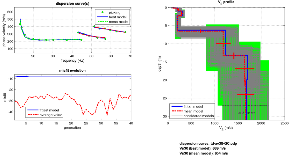
Figure 4. Inverted V_s section, from site 1 in figure 2, with the V_{s30} value. This results in a C or B ground class type soil according respectively to table 1 or table 2.
