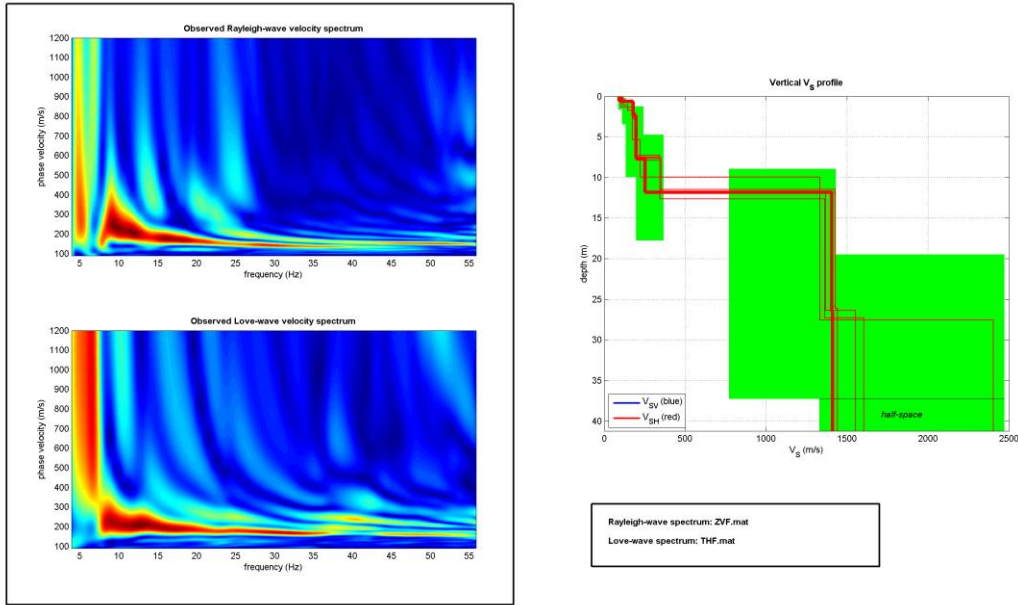
Figure 7. Inverted V_s section, from site 2 in figure 2, with a resulting V_s^{30} value of 417 m/s.
