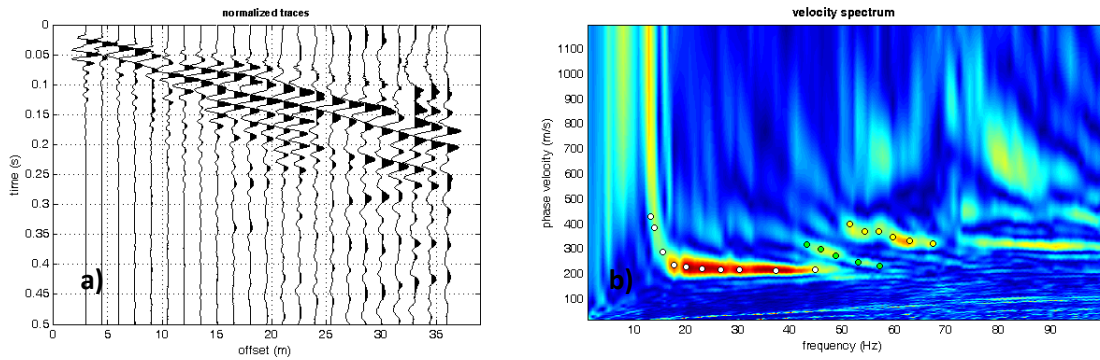
Figure 3. Multichannel shot record a) Frequency - Phase Velocity spectra with fundamental mode picking, and two additionally picked higher modes.
