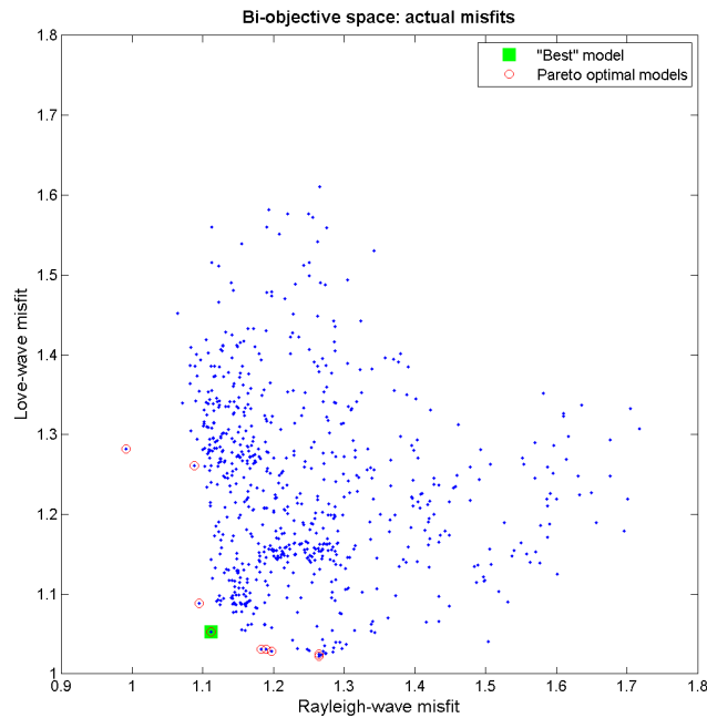
Figure 8. Pareto front models of the joint inversion of Rayleigh- and Love-wave dispersion curves. Distribution of the evaluated models in the bi-objective space (obj#1: Rayleigh-wave misfit; obj#2: Love wave misfit). Symmetry Index (S.I.) of the Pareto front models is signaled by the red circles.
