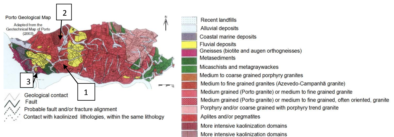
Figure 2. The Geotechnical Map of Porto along with the locations of three of the seismic dispersive surface wave tests. (Adapted from Almeida and Begonha, 2008)
