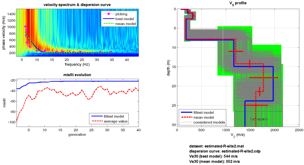
Figure 5. ReMi interpretation results section, from site 1 in figure 2, with the V_{s30} value.
